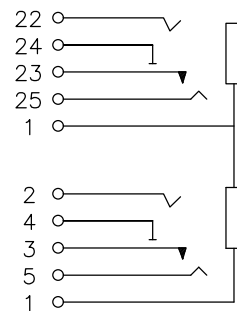
03 SCHEMATIC
