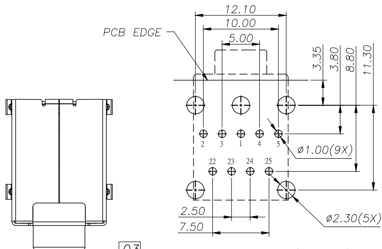
03 RECOMMENDED PCB LAYOUT(TOP VIEW) THICKNESS 1.6±0.1mm;DEFAULT TOLERANCE:±0.05
